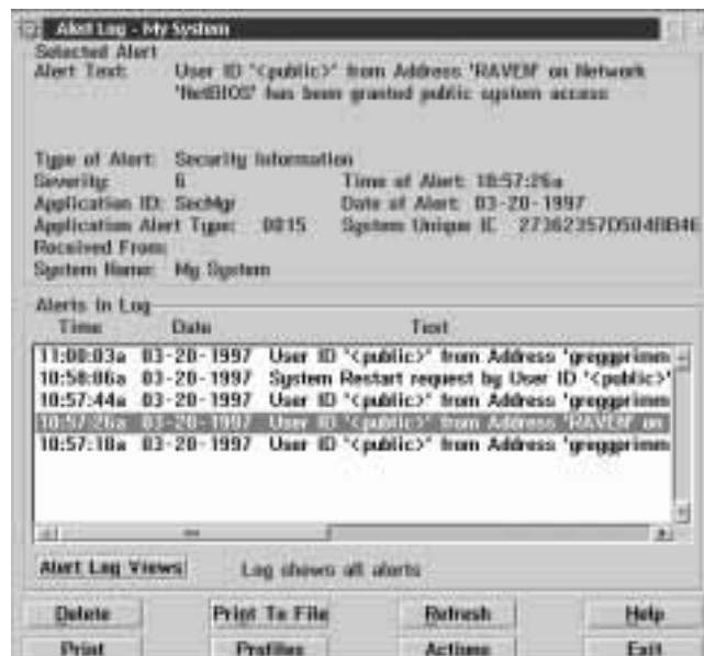
Figure 3. Alert Manager Service
